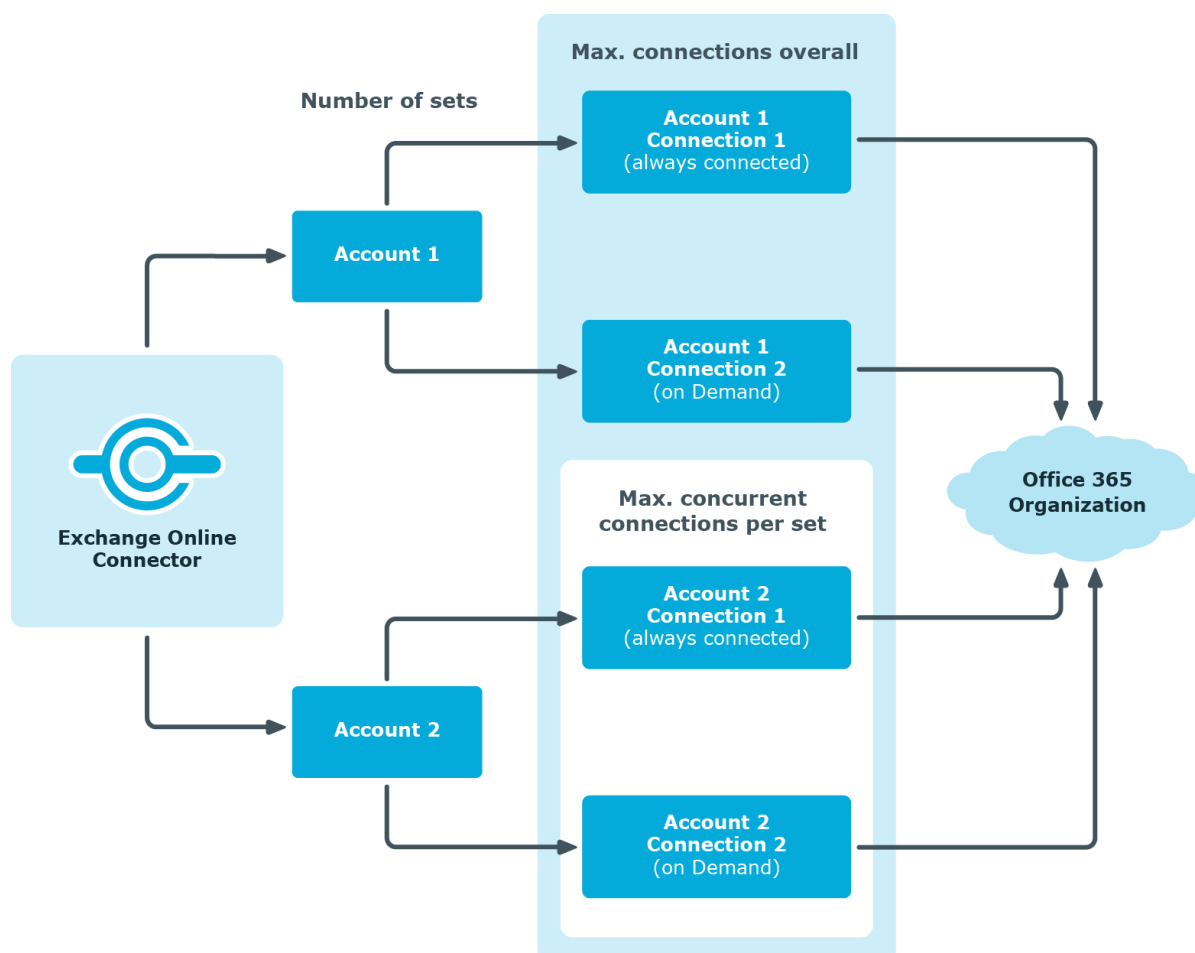
Figure 2: Determining sessions
