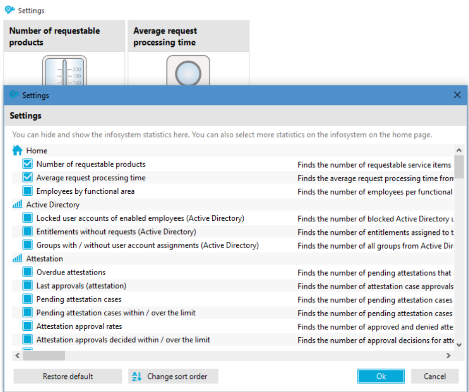
Figure 2: Statistics settings
